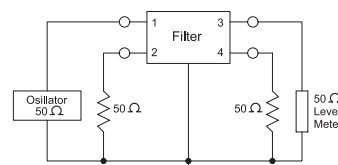
Differential Mode
