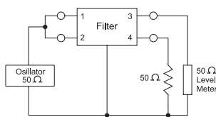
Common Mode
