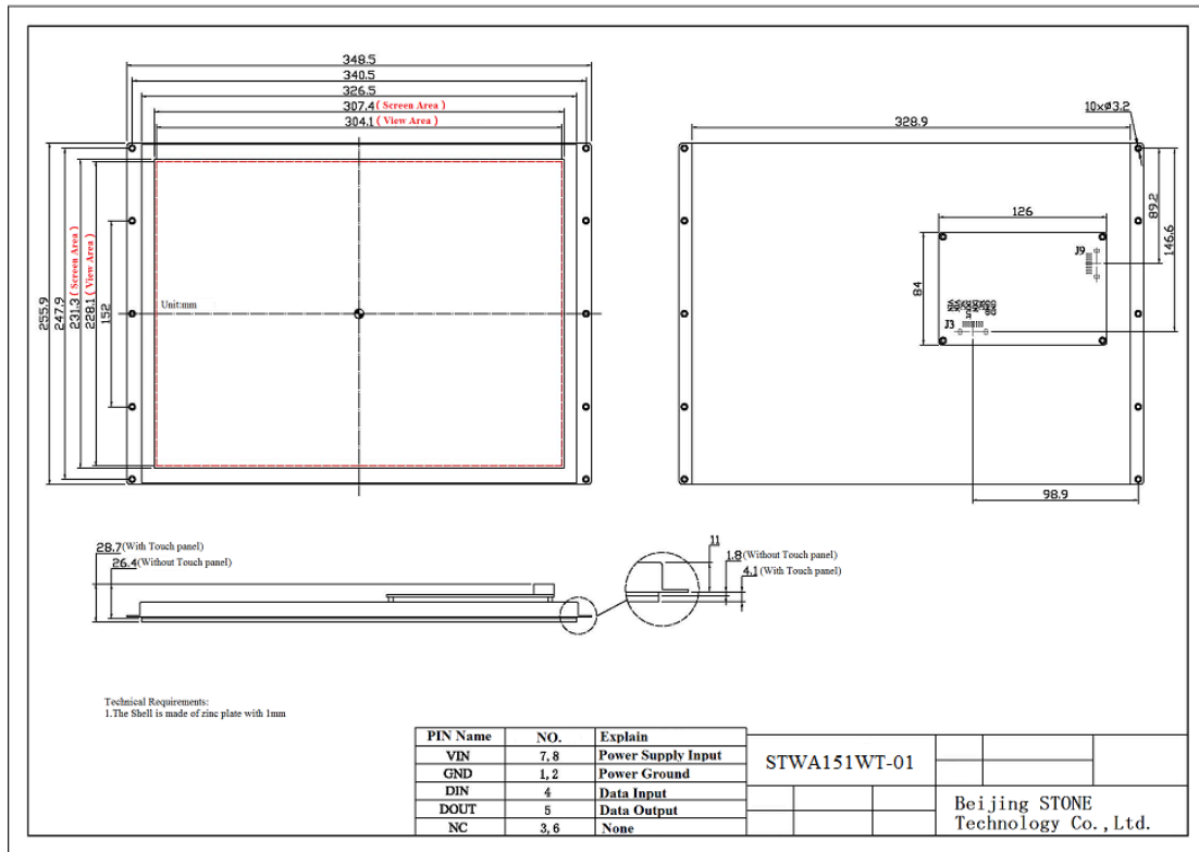
Figure 6-1 STWA151WT-01 dimension
